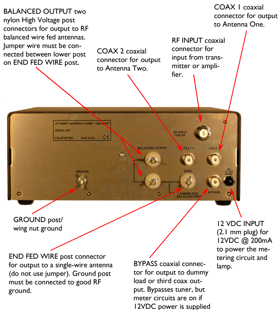
FIGURE 1 REAR PANEL CONNECTORS
