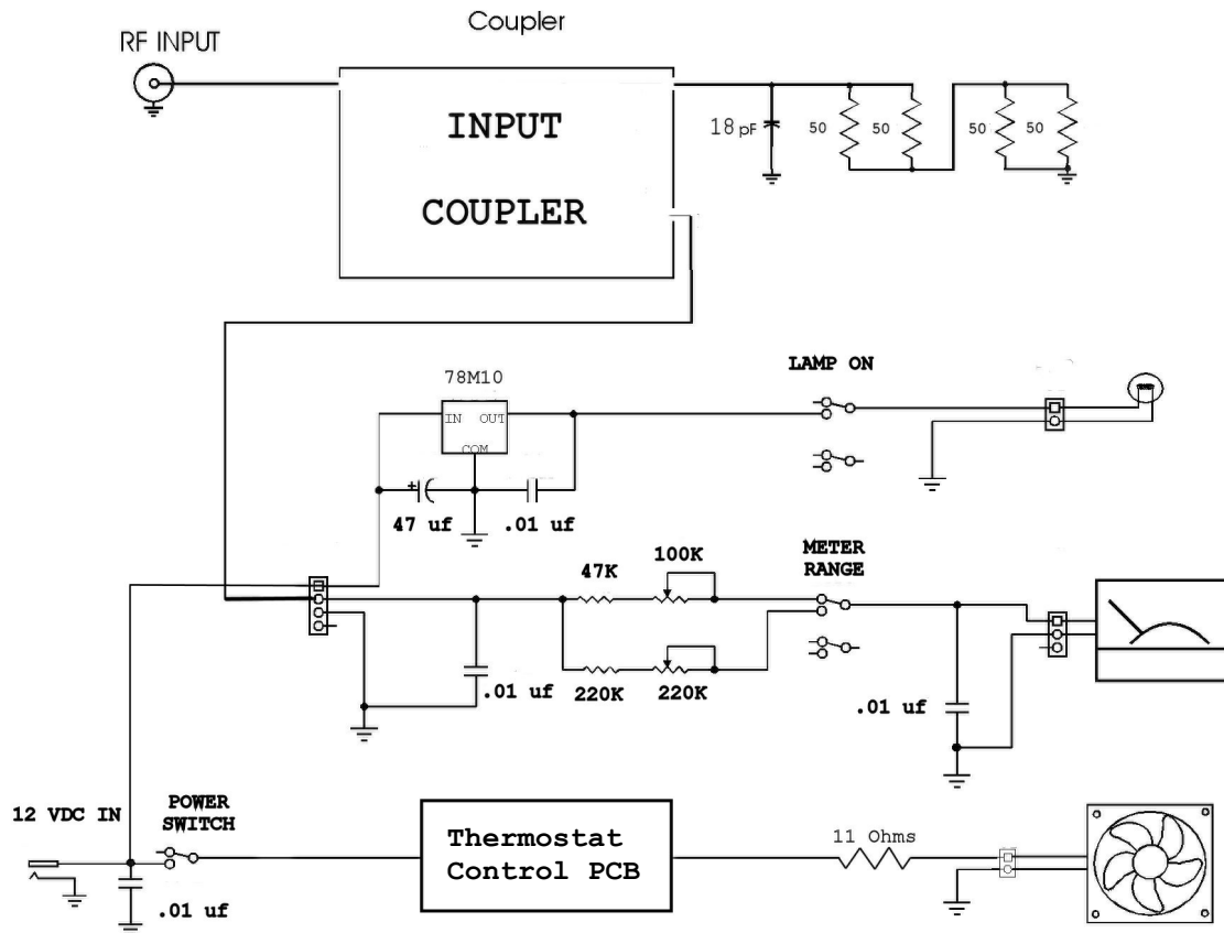
Palstar DL2K Schematic
